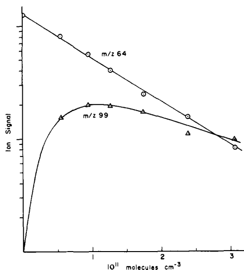
Figure 4. Semilogarithmic plot of decay of the parent ion and formation of CF 3 CH 2 O - for the reaction of 1 + CF 3 CH 2 OH. Ion signals are in arbitrary units. Formation of the cluster ion m/z 199 was omitted.
