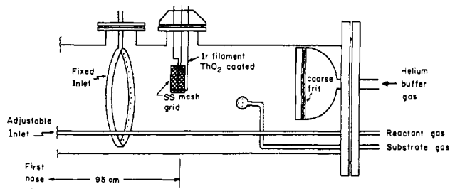
Figure 1. Ion preparation region of flowing afterglow apparatus.
